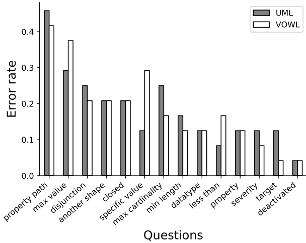
Figure 3.12: The error rates for both visual notations are relatively similar. Higher error rates for both visual notations were observed for property paths and maximum value .
